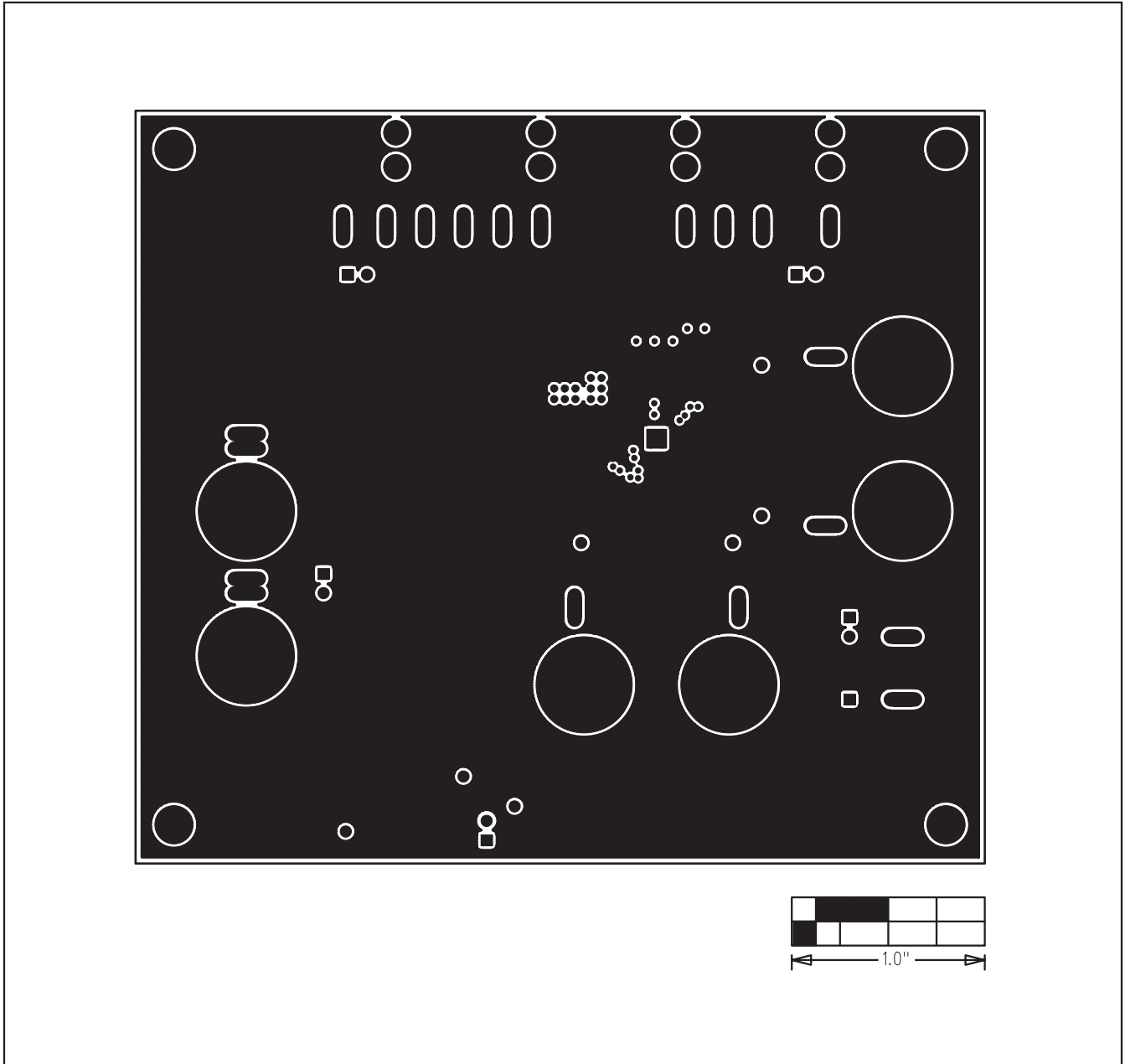
Figure 4. MAX9791A EV Kit PCB Layout—Layer 2
