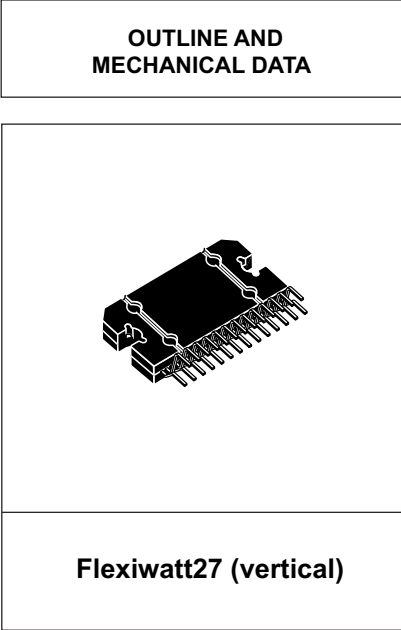
Figure 33. Flexiwatt27 (vertical) mechanical data and package dimensions
