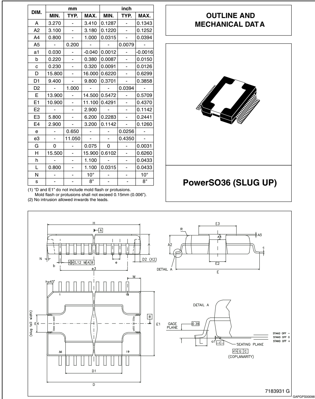
Figure 35. PowerSO36 (slug up) mechanical data and package dimensions
