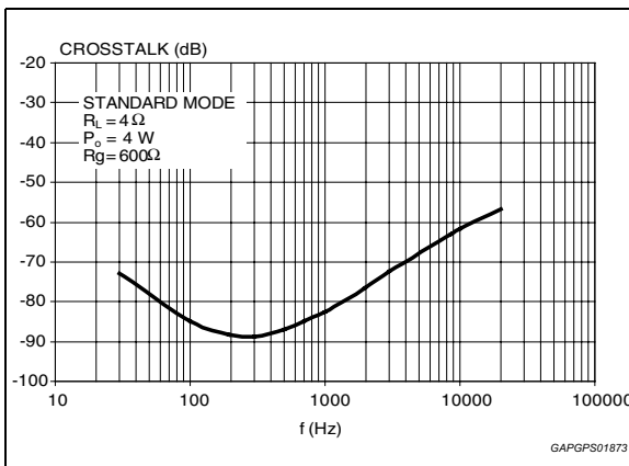
Figure 13. Crosstalk vs. frequency
