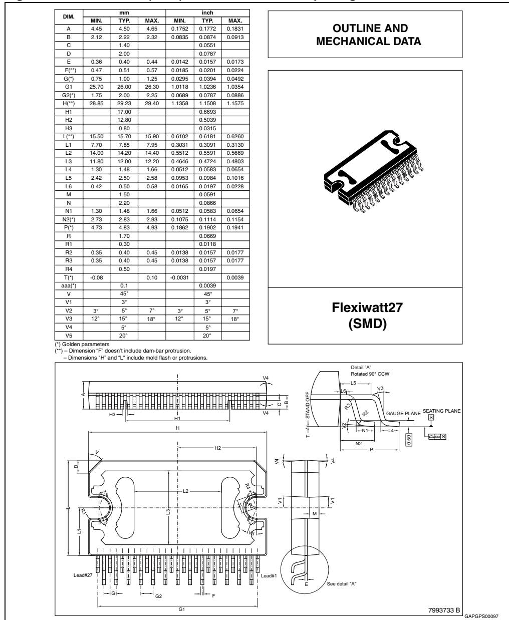
Figure 34. Flexiwatt27 (SMD) mechanical data and package dimensions
