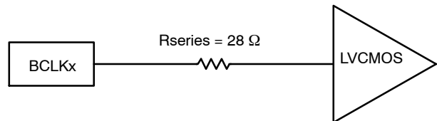
Figure 9. Series Termination
