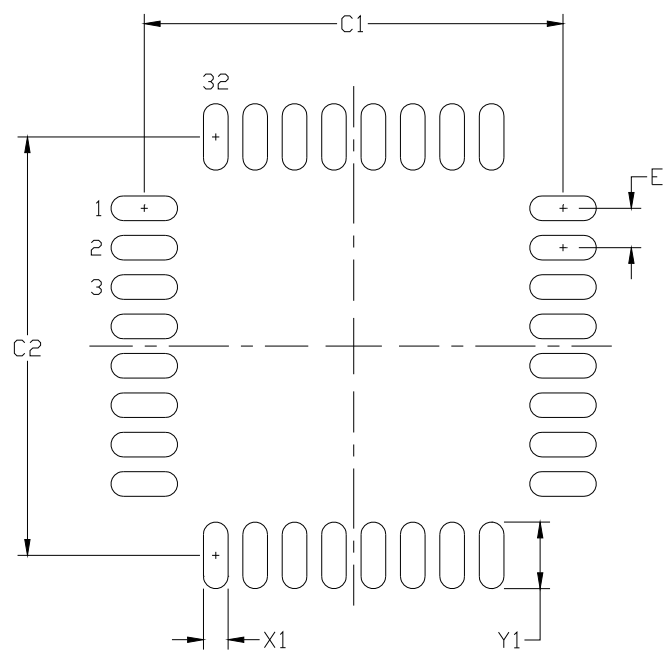
Figure 4.8. QFP-32 Package Drawing
