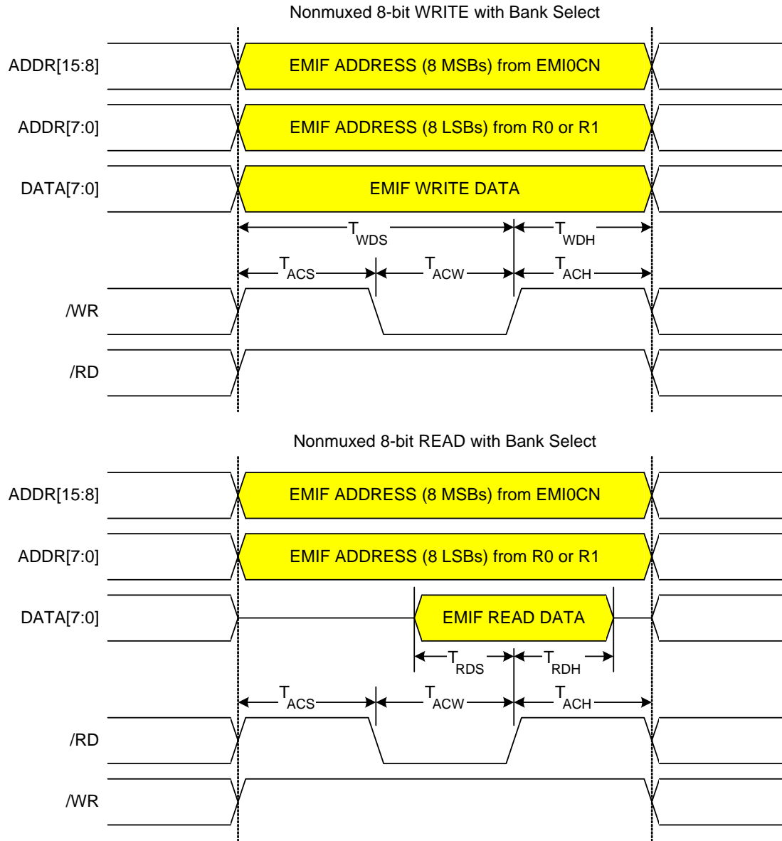
Figure 18.6. Non-multiplexed 8-bit MOVX with Bank Select Timing
