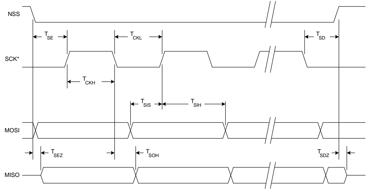
Figure 26.10. SPI Slave Timing (CKPHA = 0)
