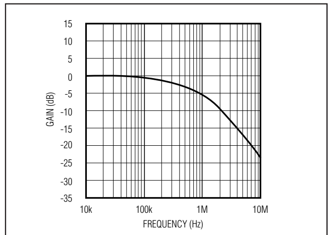
Figure 8. 1000 Feet of 24AWG Twisted-Pair Telephone Cable (Gain vs. Frequency)
