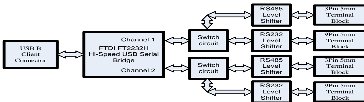
Figure 1.2 USB2-H-9002-M Block Diagram
