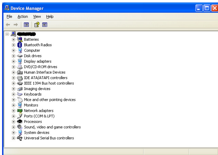
Figure 2.9 - Device Manager
