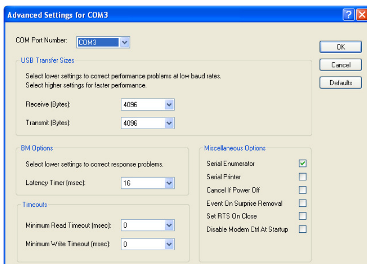
Figure 2.13 - Advanced Options
