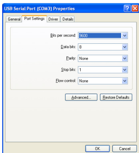
Figure 2.12 - Settings Tab
