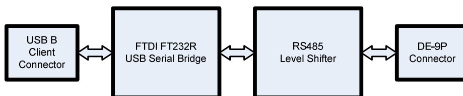
Figure 1.2 USB2-F-5001 Block Diagram
