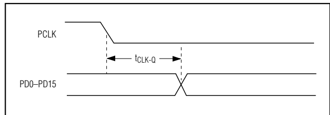
Figure 2. Timing Parameters
