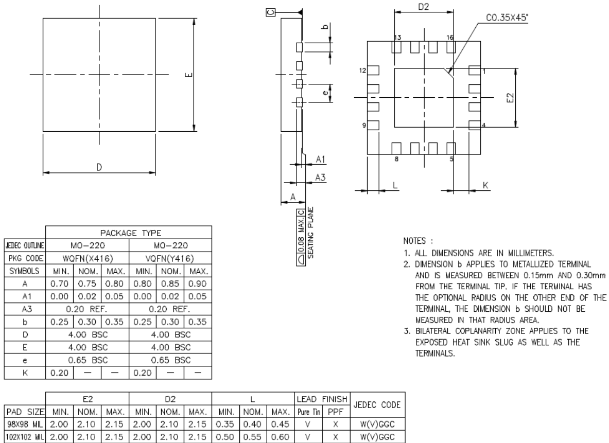
Figure 9.3 QFN-16 Package Dimensions
