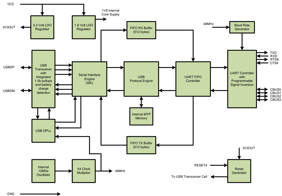
Figure 2.1 FT230X Block Diagram
