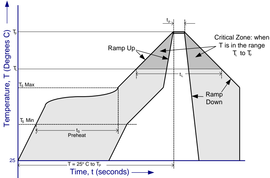
Figure 9.5 FT230X Solder Reflow Profile
