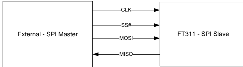
Figure 5-4 SPI Slave block diagram
