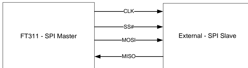
Figure 5-5 SPI Master block diagram
