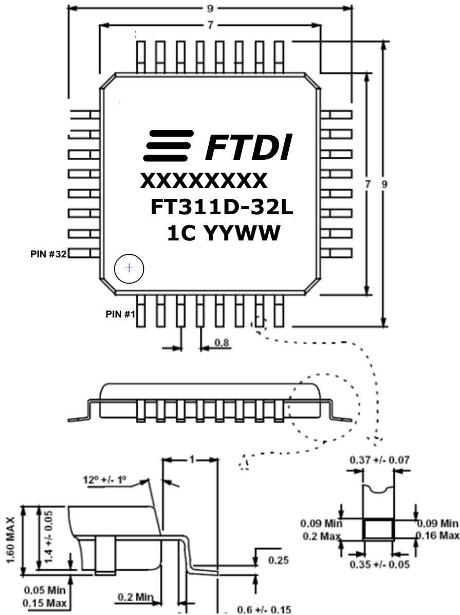
Figure 9-4 LQFP-32 Package Dimensions
