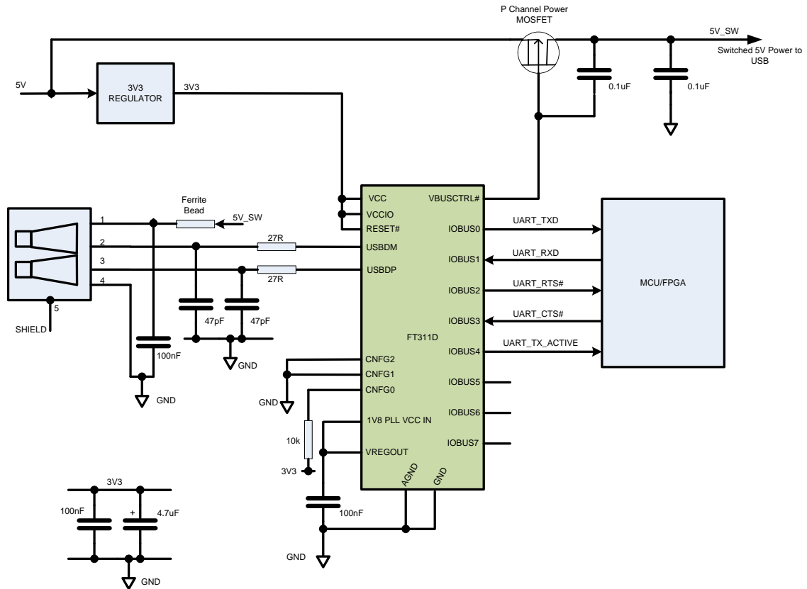
Figure 8.2 Application Example showing USB to UART Converter
