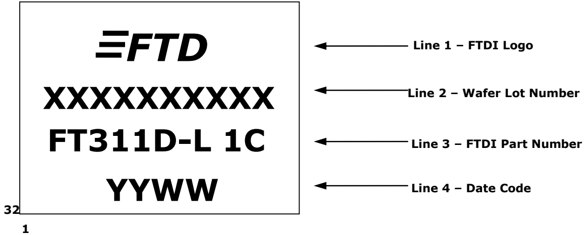
Figure 9-2 LQFP Package Markings
