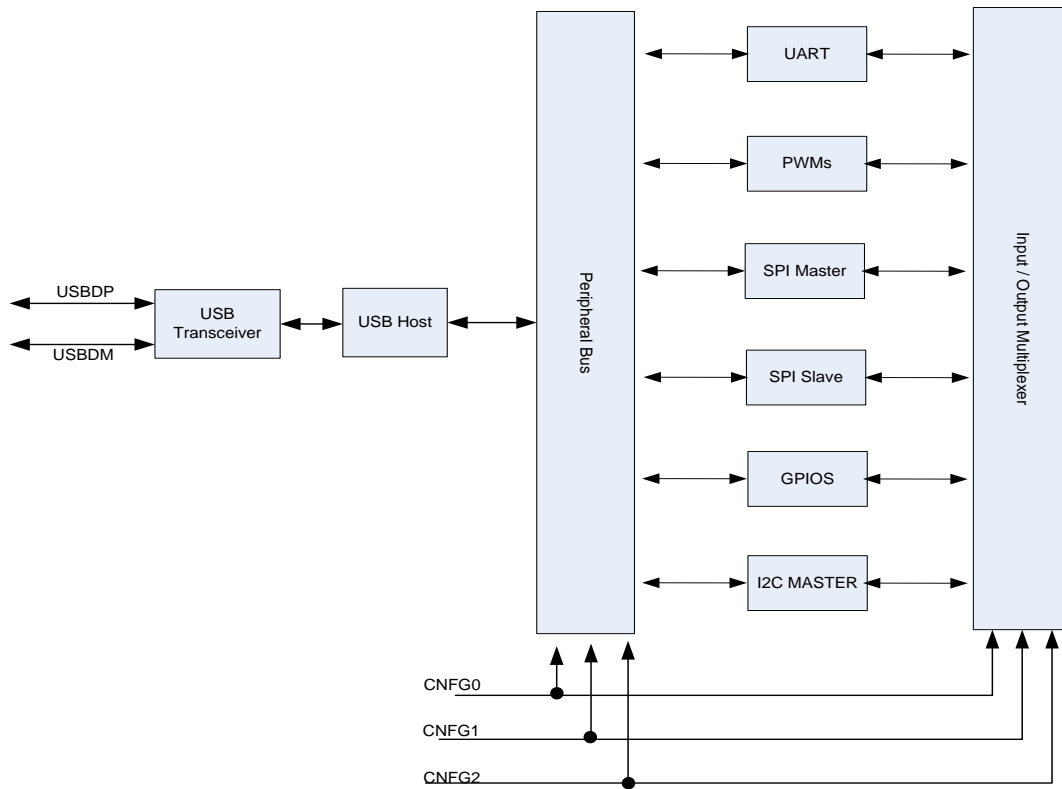
Figure 2.1 FT311D Block Diagram
