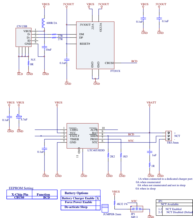
Figure 8.2 USB Battery Charging Detection (1- pin)
