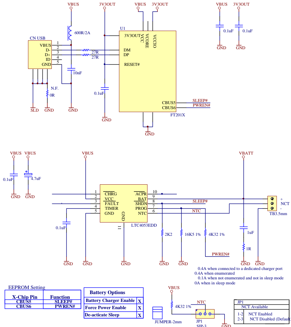
Figure 8.3 USB Battery Charging Detection (2- pin)
