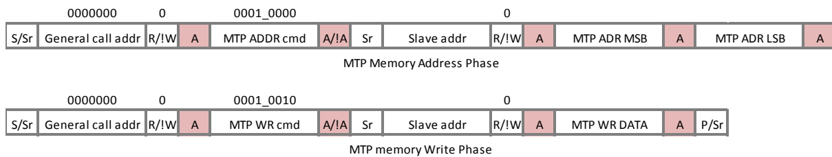
Figure 10.2: Write EEPROM command sequence
