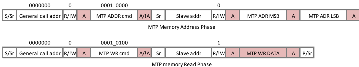
Figure 10.3: Read EEPROM command sequence
