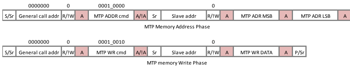
Figure 10.2 Write EEPROM command sequence
