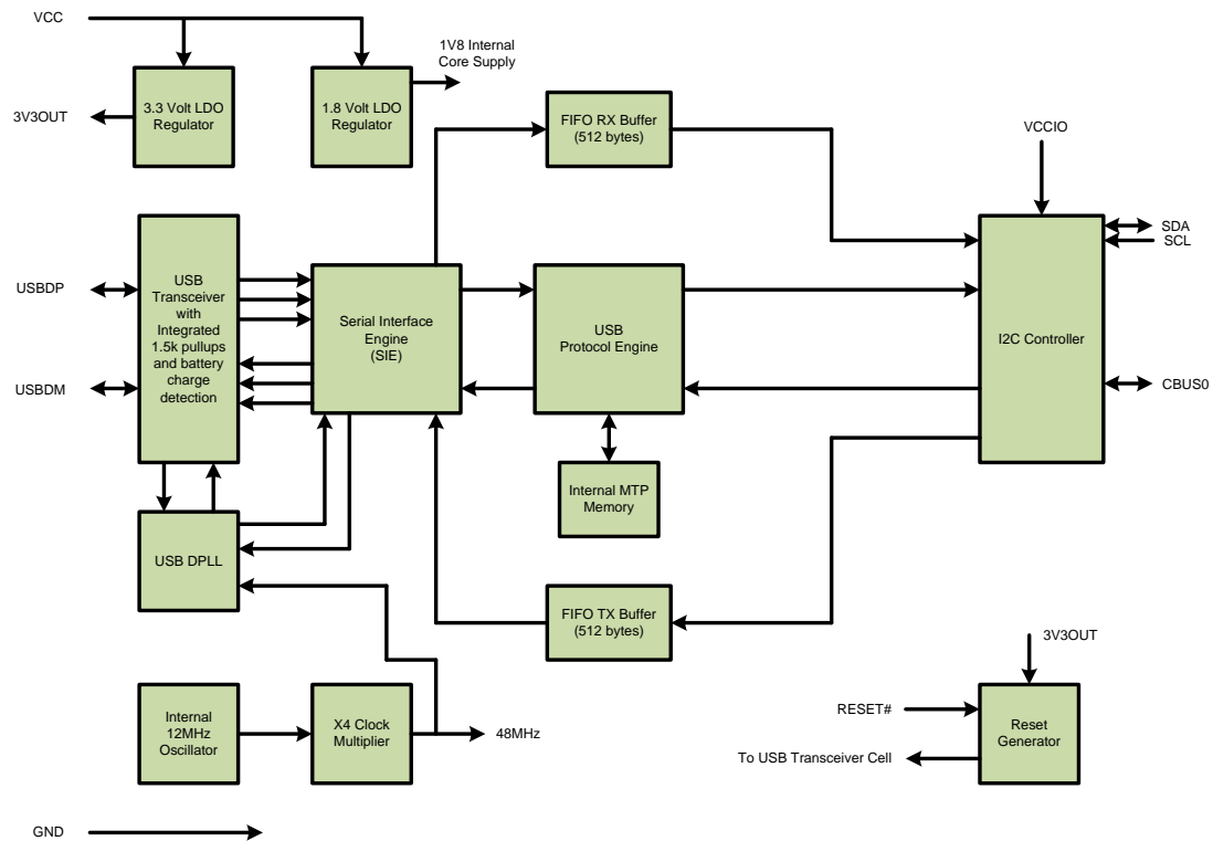
Figure 2.1FT200XD Block Diagram
