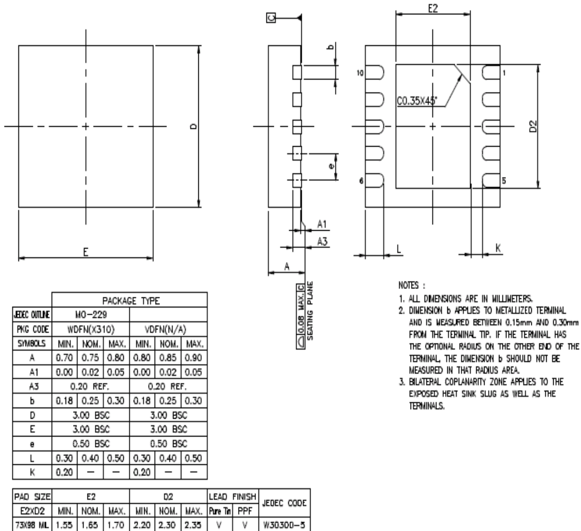
Figure 11.1 DFN-10 Package Dimensions
