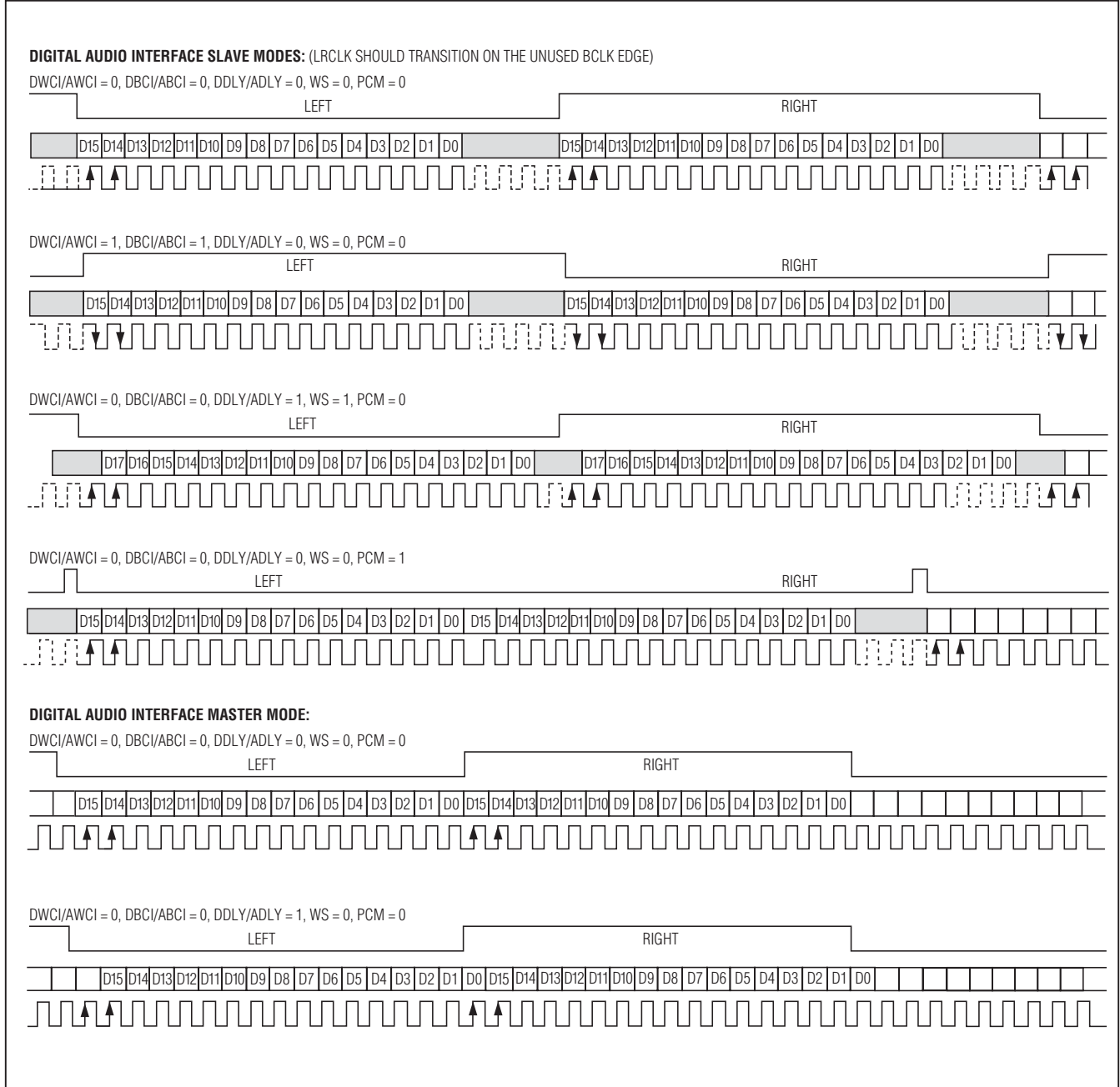
Figure 1. Digital Audio Interface Data Format Examples
