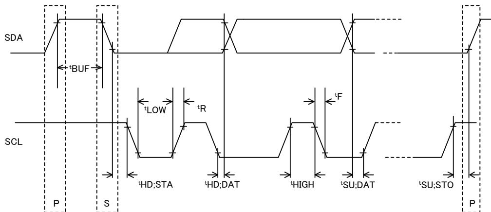
Figure VI.11.5 Timing chart
