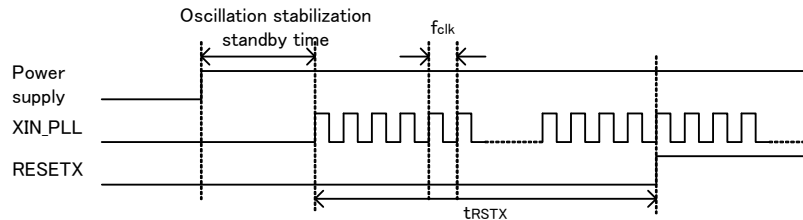
Figure VI.1 Reset Timing
