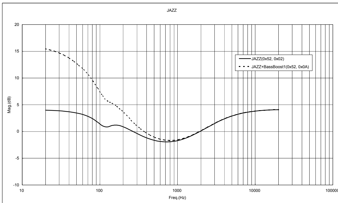
Figure VII.3.3.2 JAZZ Frequency Characteristics
