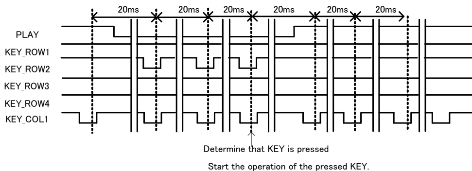
Figure VII.2.2 Operating Waveforms when KEY is Pressed
