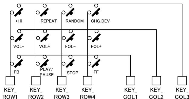
Figure VI.10 KEY Matrix Applied Circuit Diagram
