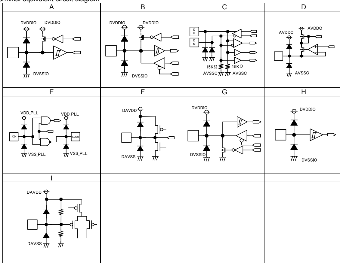
I/O terminal equivalent circuit diagram
