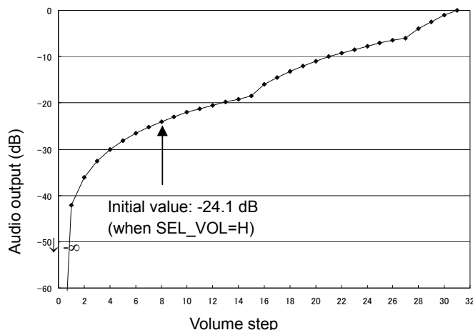
Figure VI.5 Volume Step Function
