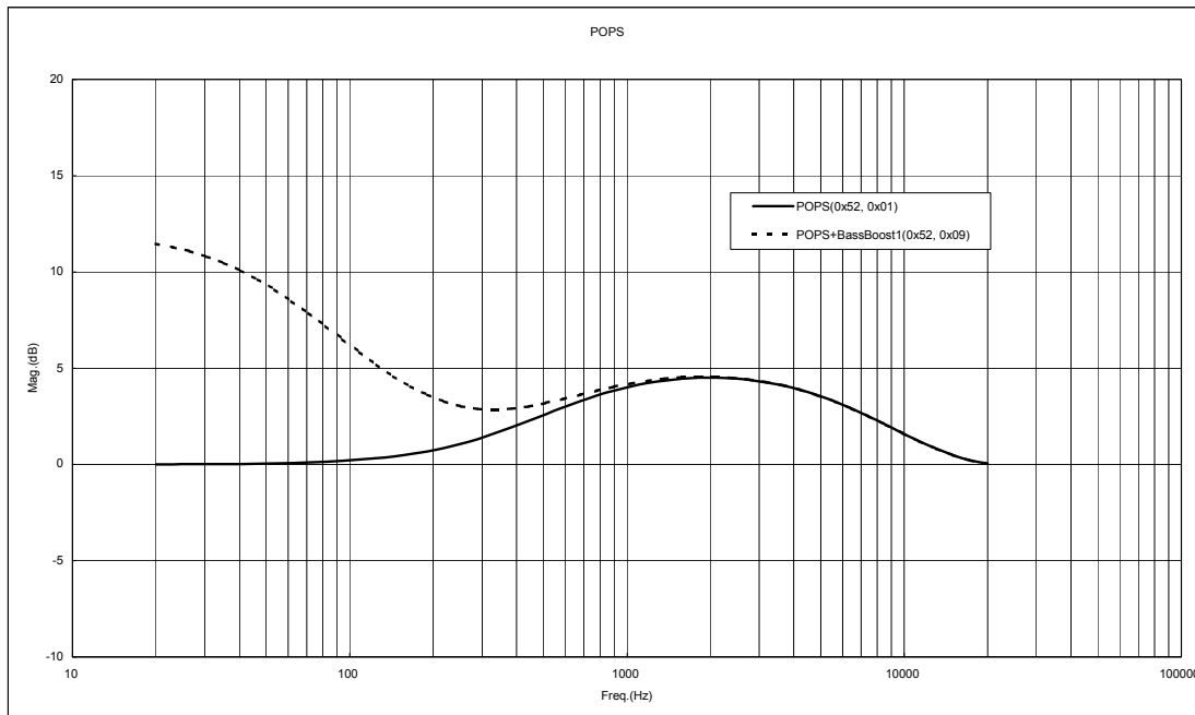
Figure VII.3.3.1 POPS Frequency Characteristics
