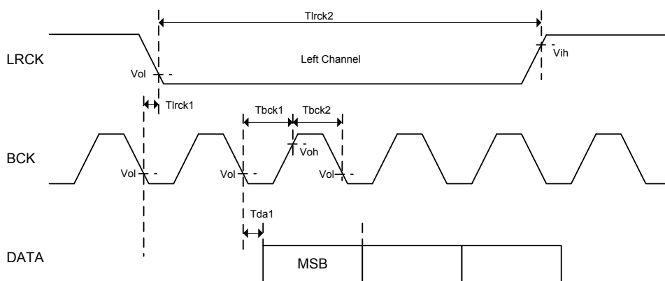
Figure VI.12.4 Timing chart
