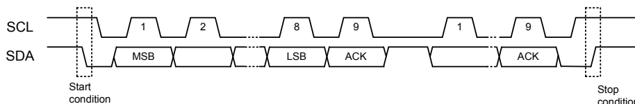
Figure VI.11.1 I 2 C start, stop condition
