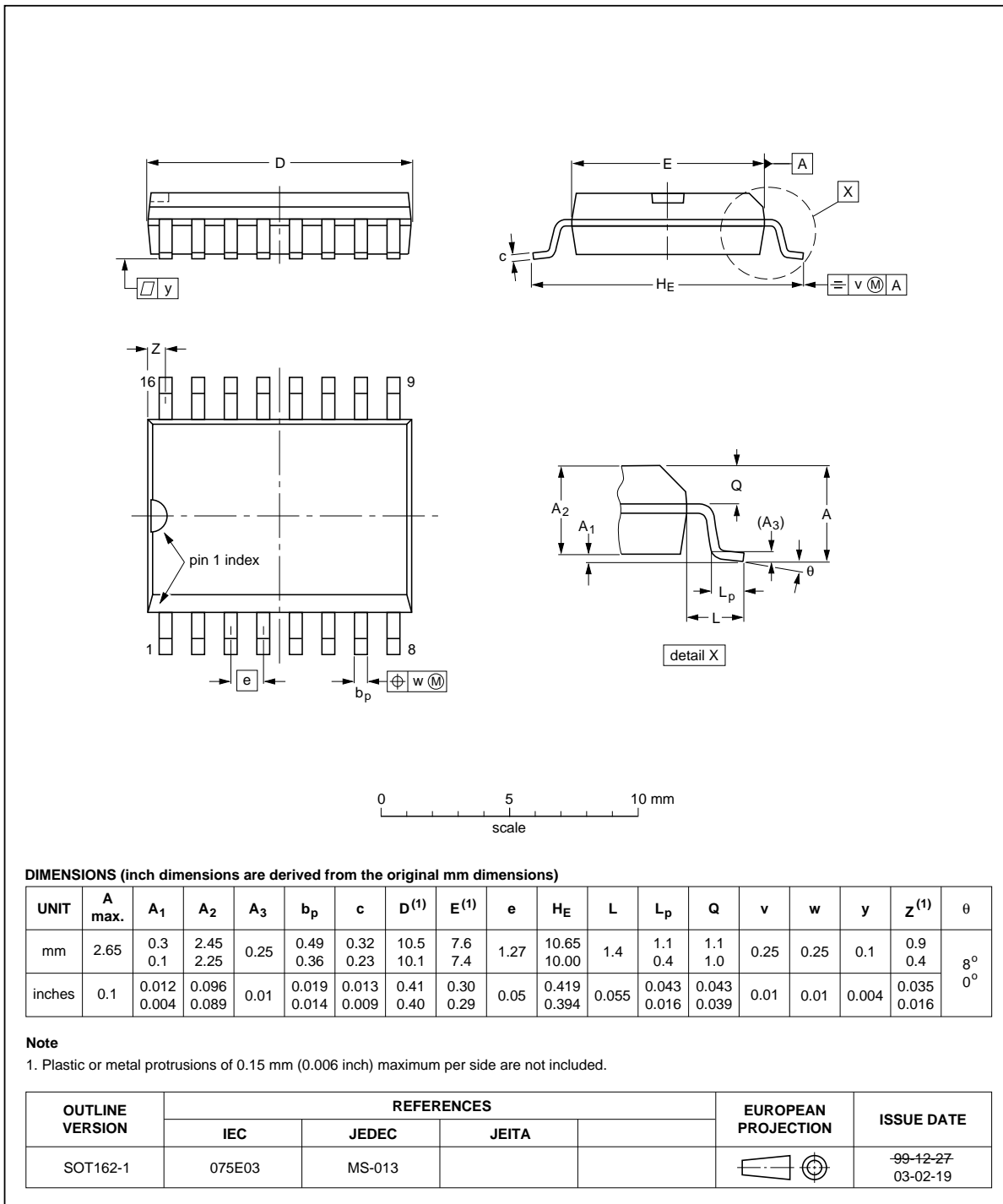
Fig 17. Package outline SOT162-1 (SO16)
