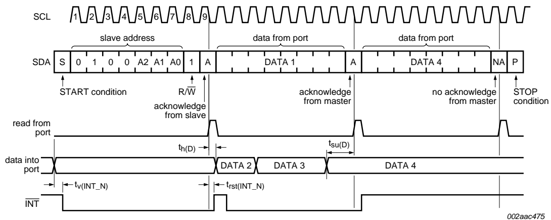
Fig 13. Read from register
