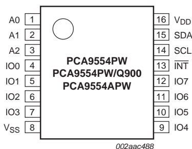
Fig 4. Pin configuration for TSSOP16
