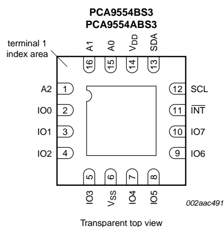
Fig 7. Pin configuration for HVQFN16 (SOT758-1)
