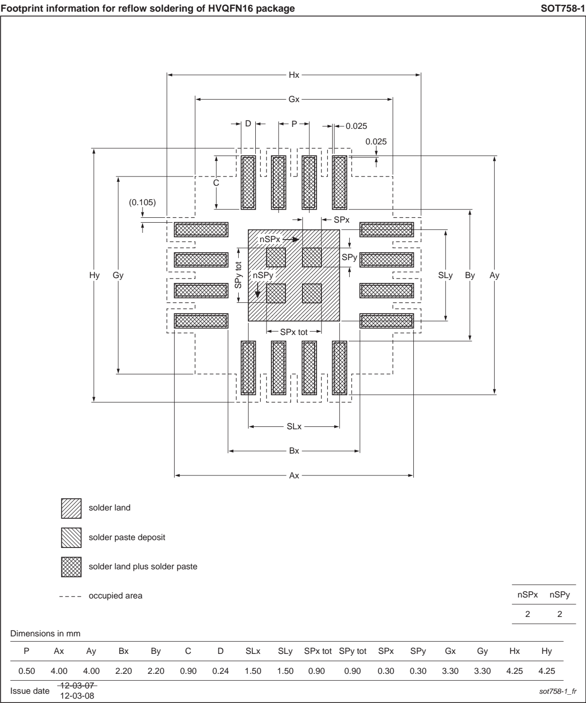
Fig 29. PCB footprint for SOT758-1 (HVQFN16); reflow soldering
