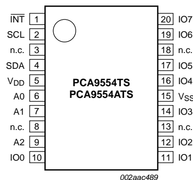
Fig 5. Pin configuration for SSOP20
