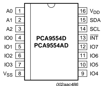
Fig 2. Pin configuration for SO16
