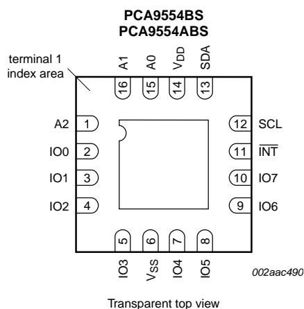
Fig 6. Pin configuration for HVQFN16 (SOT629-1)
