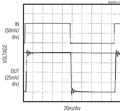
SMALL-SIGNAL PULSE RESPONSE ( A_{vCL} = 1 )
