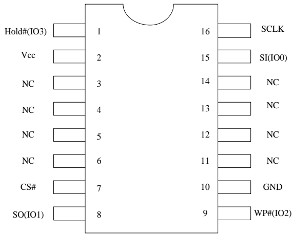
16-Pin SOIC
