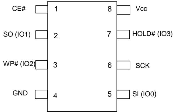
8-Pin SOIC/SOP
