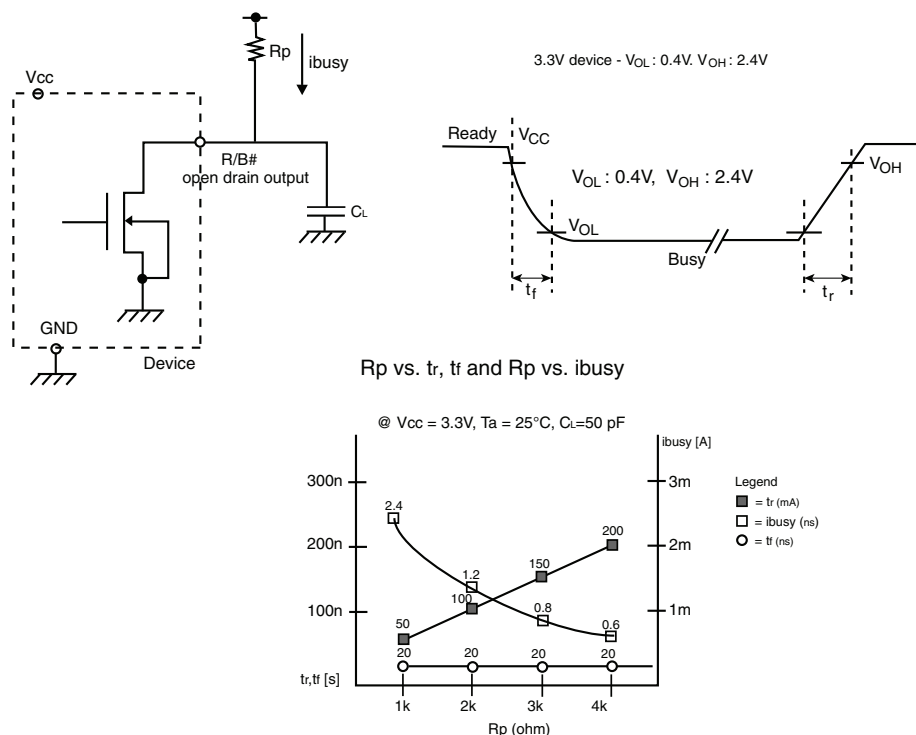
Figure 4.1 Ready/Busy Pin Electrical Application
