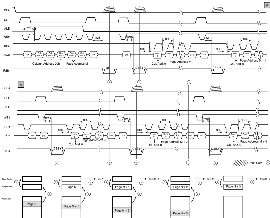
Figure 6.27 Read Cache Operation Timing
