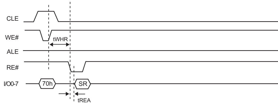
Figure 6.24 Read Status Timing
