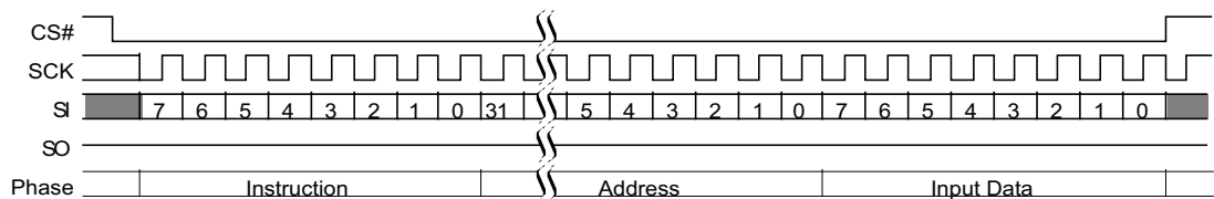
Figure 10.64 DYBWR (E1h) Command Sequence
