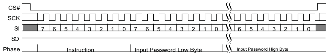
Figure 10.72 Password Unlock (PASSU E9h) Command Sequence
