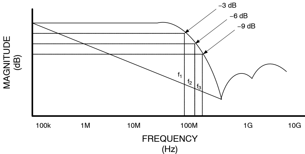
Figure 4. Filter Bandwidth
