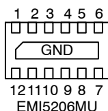
Figure 3. Pin Diagram (Bottom View)
