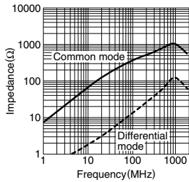
ACM2520-301-2P
