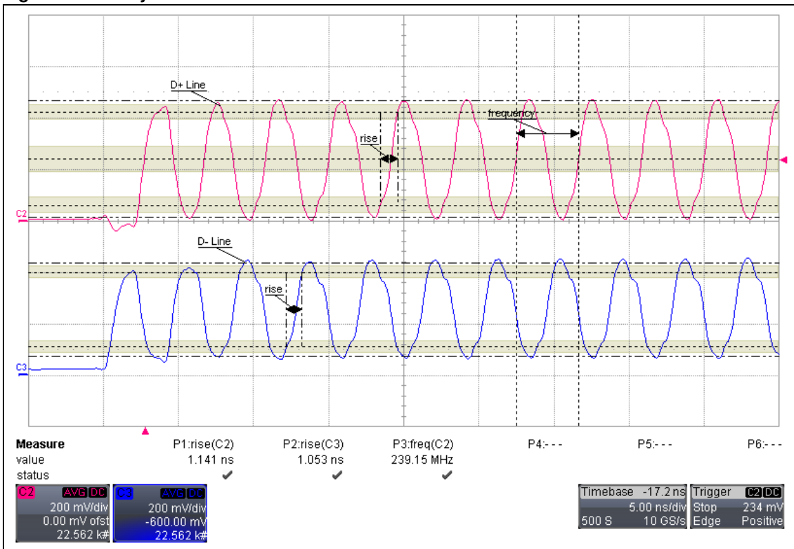
Figure 16. HS sync
