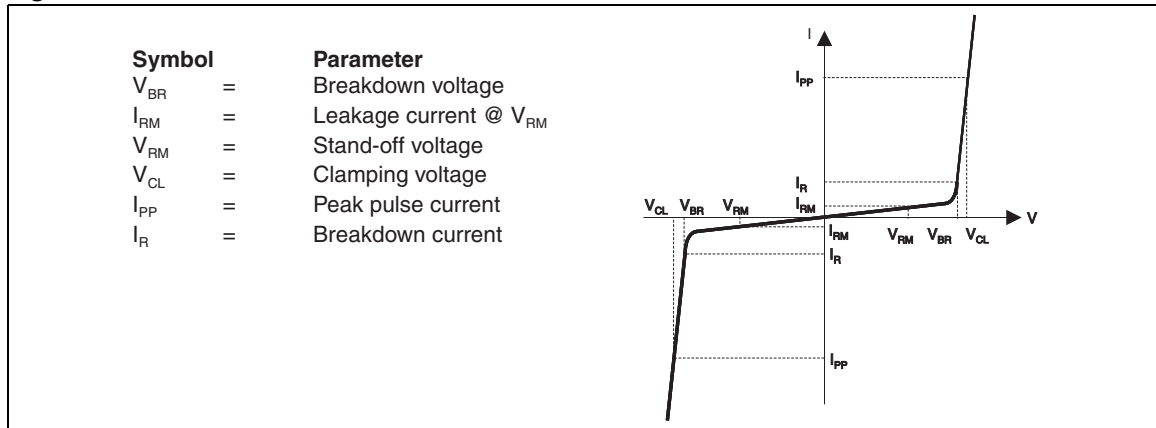
Figure 2. Electrical characteristics - definitions
