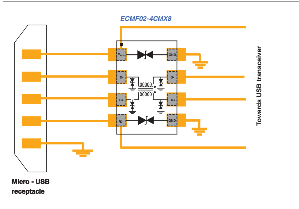
Figure 19. Application schematic
