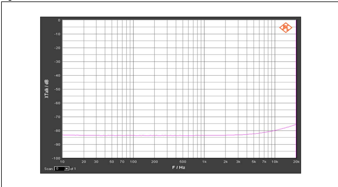
Figure 18. Crosstalk on differential lanes
