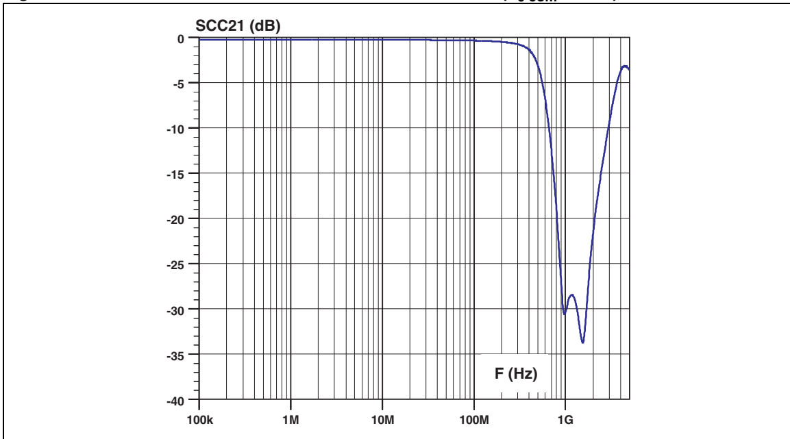
Figure 5. ID frequency response measurement ( Z_0 = 75 \Omega )
