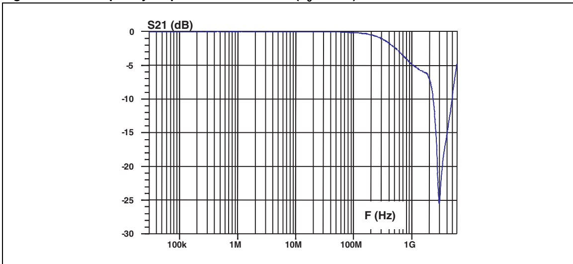
Figure 5. ID frequency response measurement ( Z_0 = 75 \Omega )
