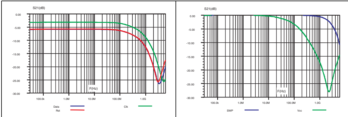
Figure 4. Attenuation measurements C1-C3, Figure 5. Attenuation measurements A1-C2 A2-A3, B1-B3
