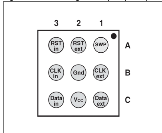
Figure 1. Pin configuration (bump side)
