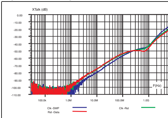
Figure 6. Analog Xtalk measurements
