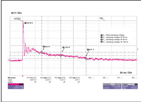
Figure 14. ESD response to IEC 61000-4-2 (+8 kV contact discharge) SWP line
