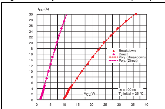
Figure 8. Dynamic characteristic (SWP)
