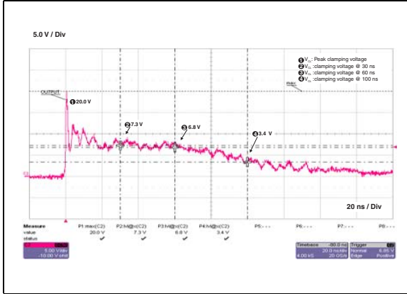
Figure 10. ESD response to IEC 61000-4-2 (+8 kV contact discharge) CLK line
