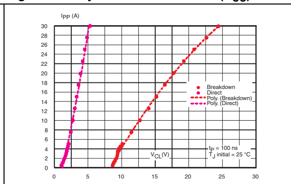
Figure 9. Dynamic characteristic (VCC)
