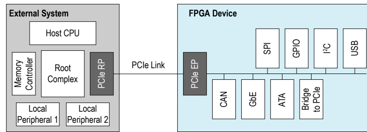
Figure 9: PCIe Multifunction for Cyclone V Devices
