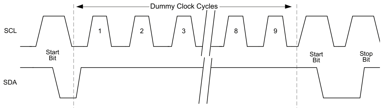
Figure 5-1. Software Reset
