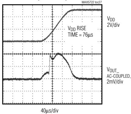
POWER-ON RESET, SLOW RISE TIME ( V_{DD} = +5V )
