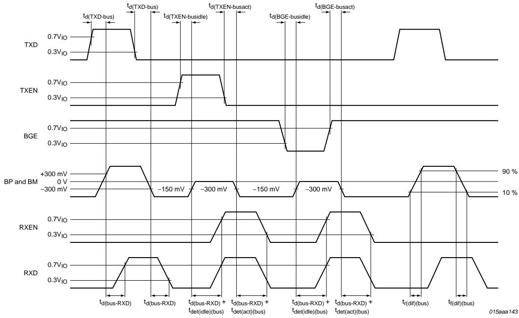
Fig 12. Detailed timing diagram in node configuration
