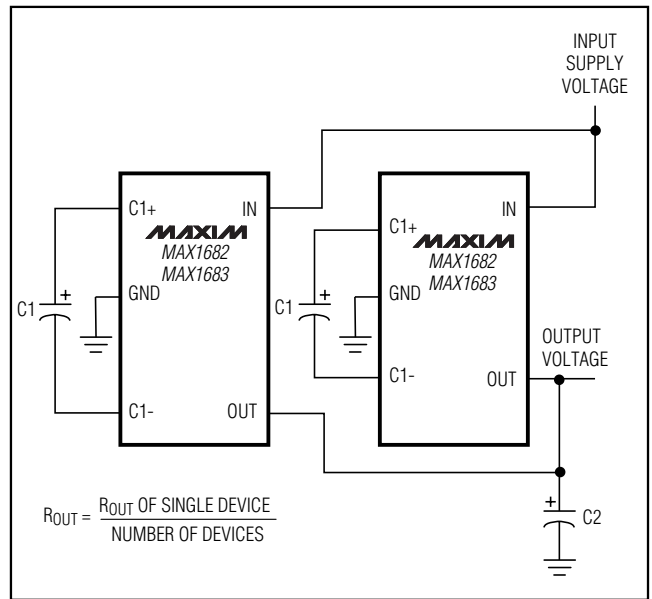
Figure 4. Paralleling Devices
