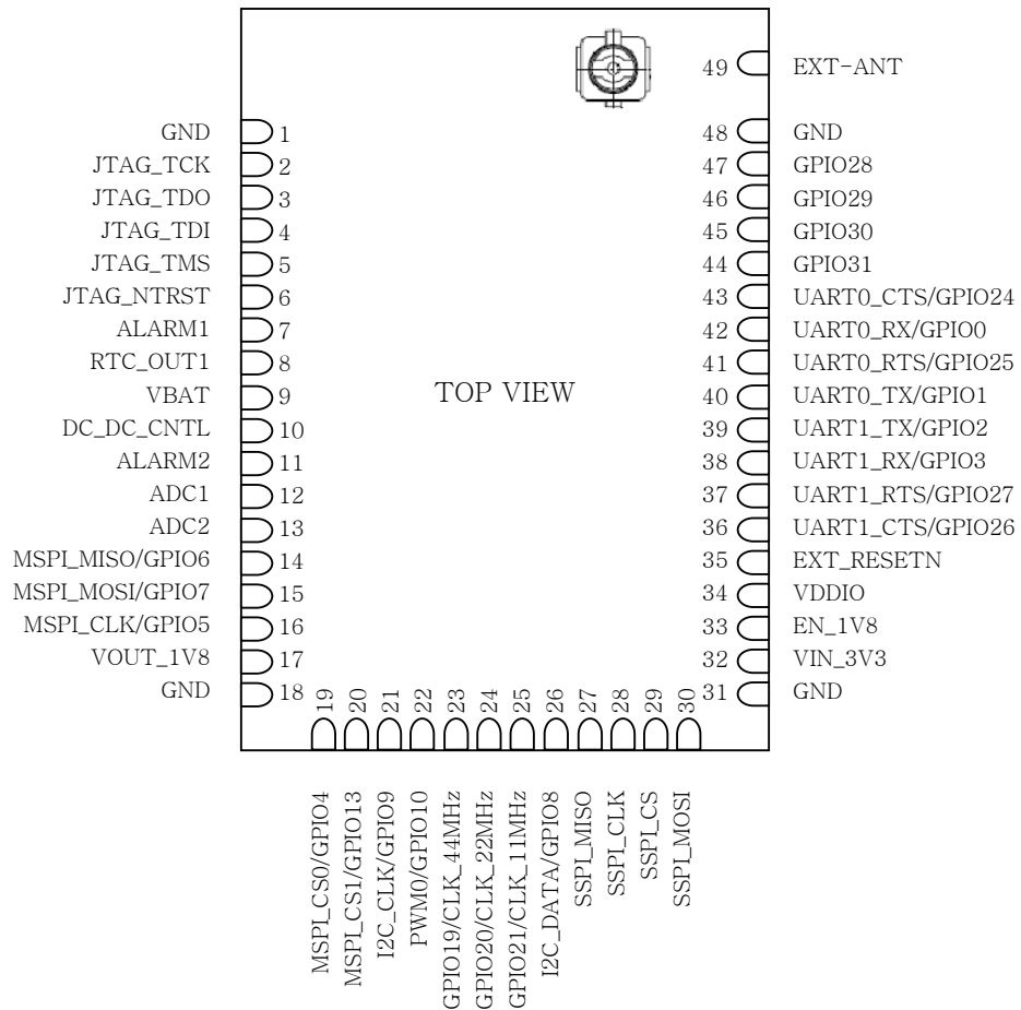
Figure 3. Pin description
