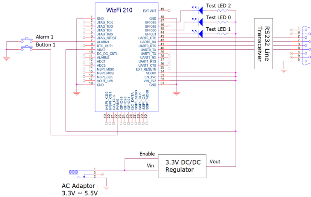
Figure 8. AC Adaptor, always ON
