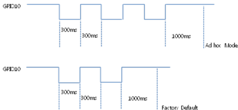
Figure 11. Factory Default and ad hoc mode
