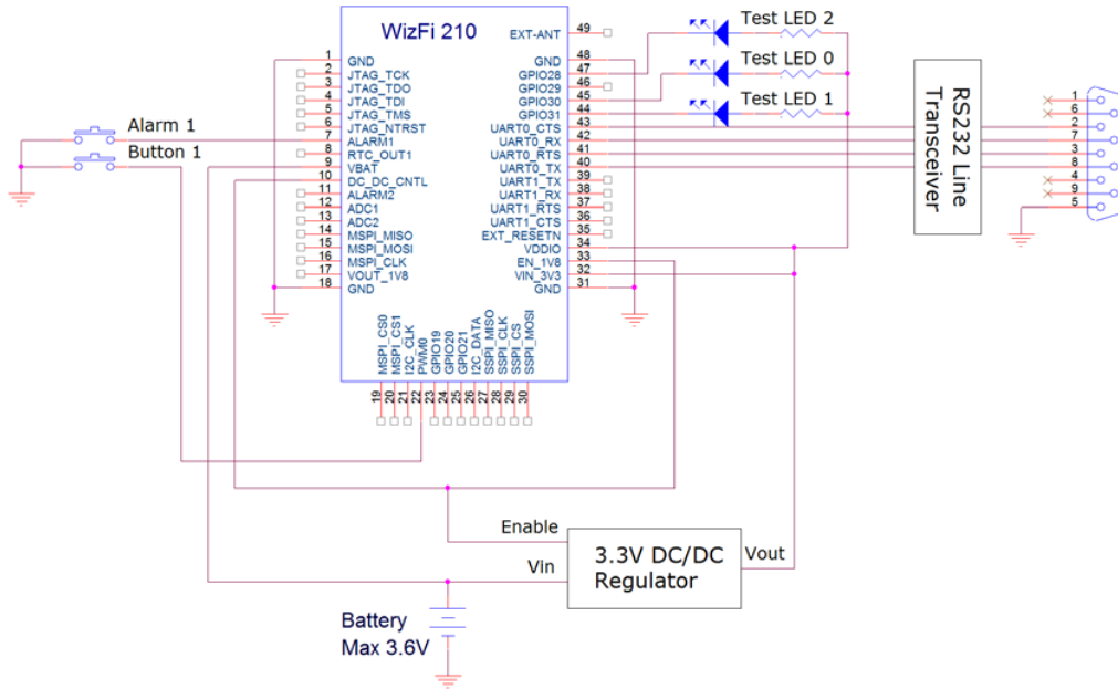
Figure 6. V_{IN} = Battery, Standby support
