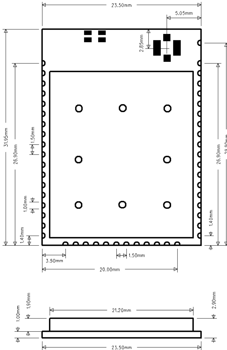
Figure 4. Module dimension
