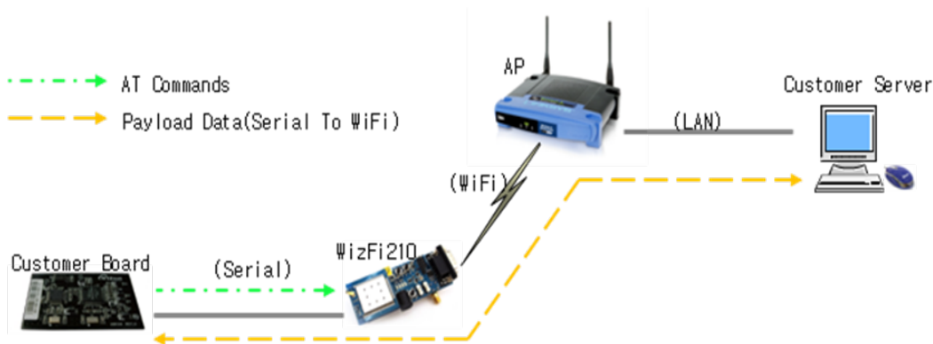
Figure 1. Basic Diagram
