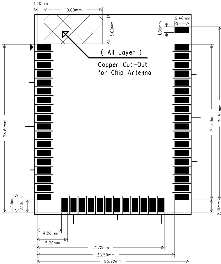
Figure 5. Recommend Pad Dimension
