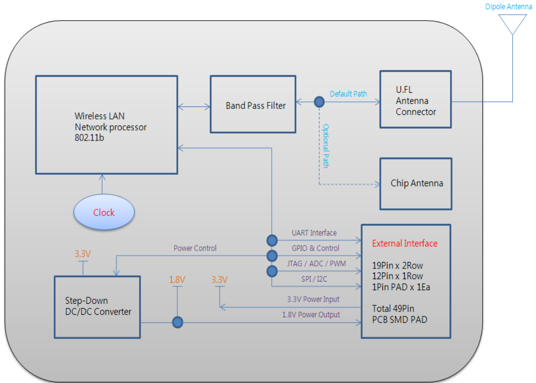
Figure 2. Block Diagram
