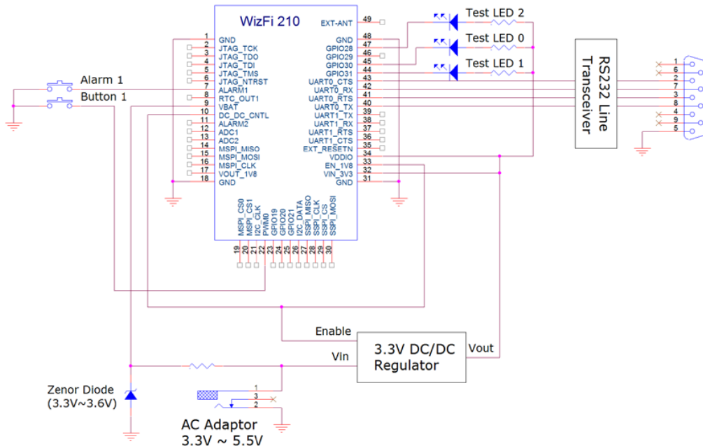
Figure 7. V_{IN} = AC Adaptor, Standby support
