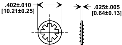
LOCK WASHER
