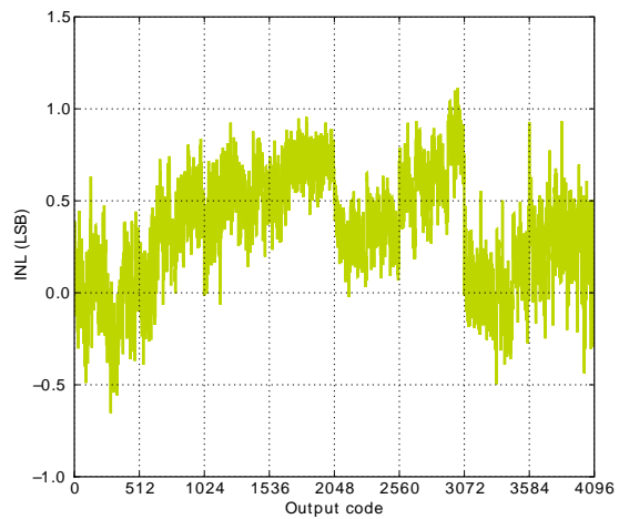
2.5V Reference
