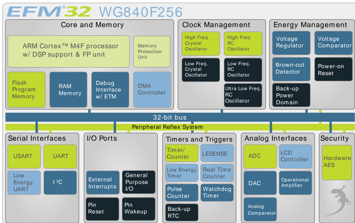
Figure 2.1. Block Diagram
