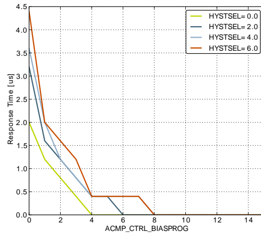
Response time
