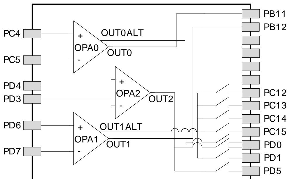
Figure 4.2. Opamp Pinout
