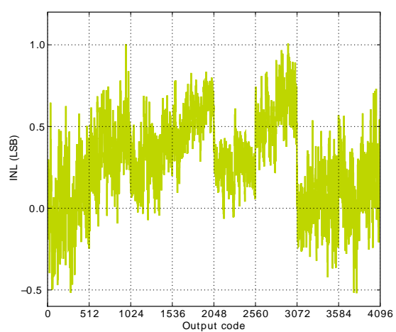
5VDIFF Reference
