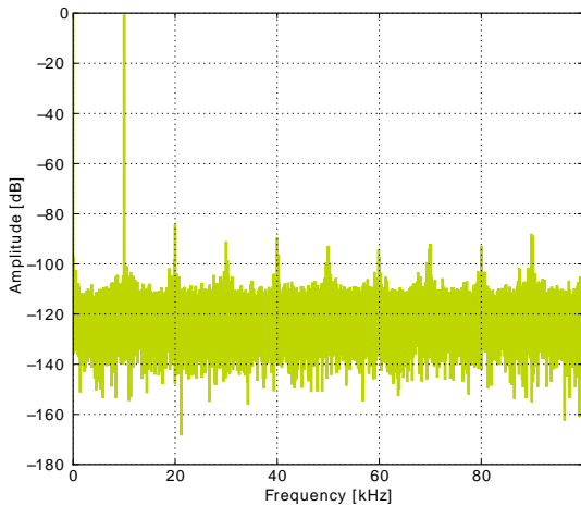
2XVDDVSS Reference
