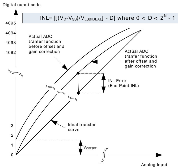
Figure 3.13. Integral Non-Linearity (INL)
