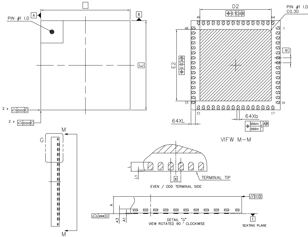
Figure 4.3. QFN64
