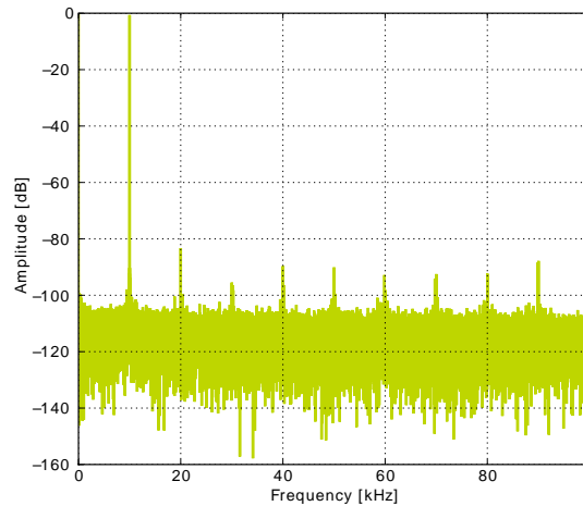
5VDIFF Reference
