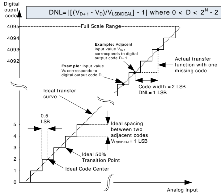
Figure 3.14. Differential Non-Linearity (DNL)
