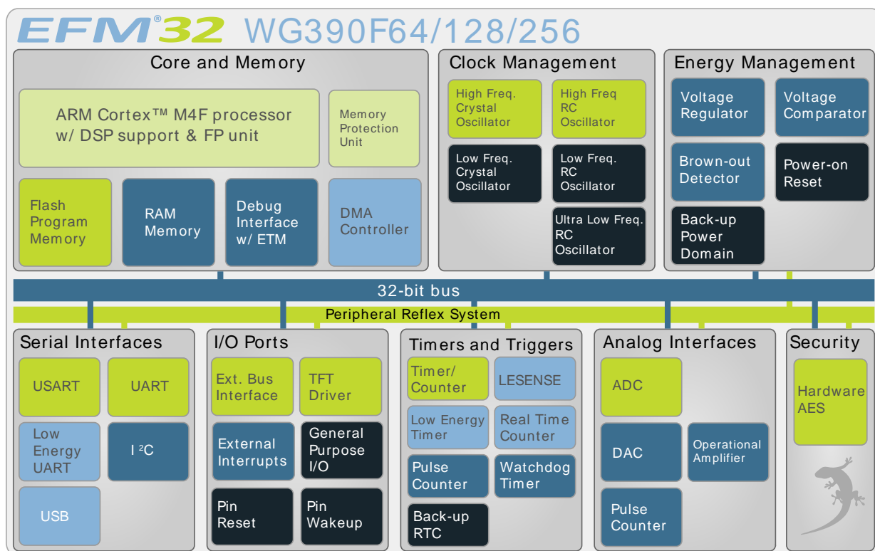
Figure 2.1. Block Diagram
