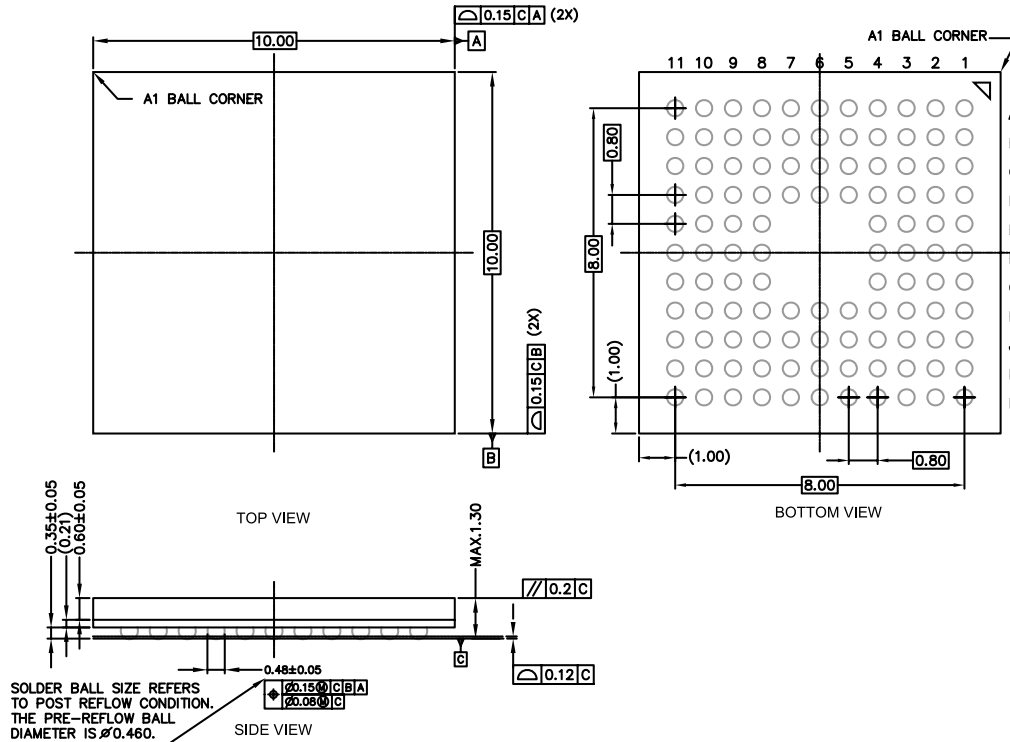
Figure 4.3. BGA112
