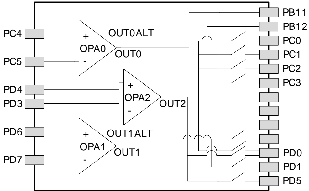
Figure 4.2. Opamp Pinout
