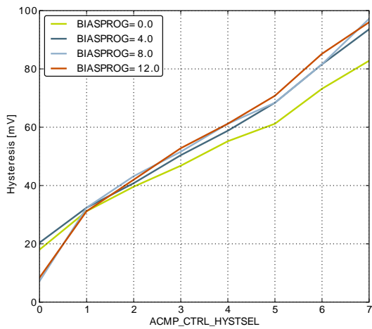
Hysteresis
