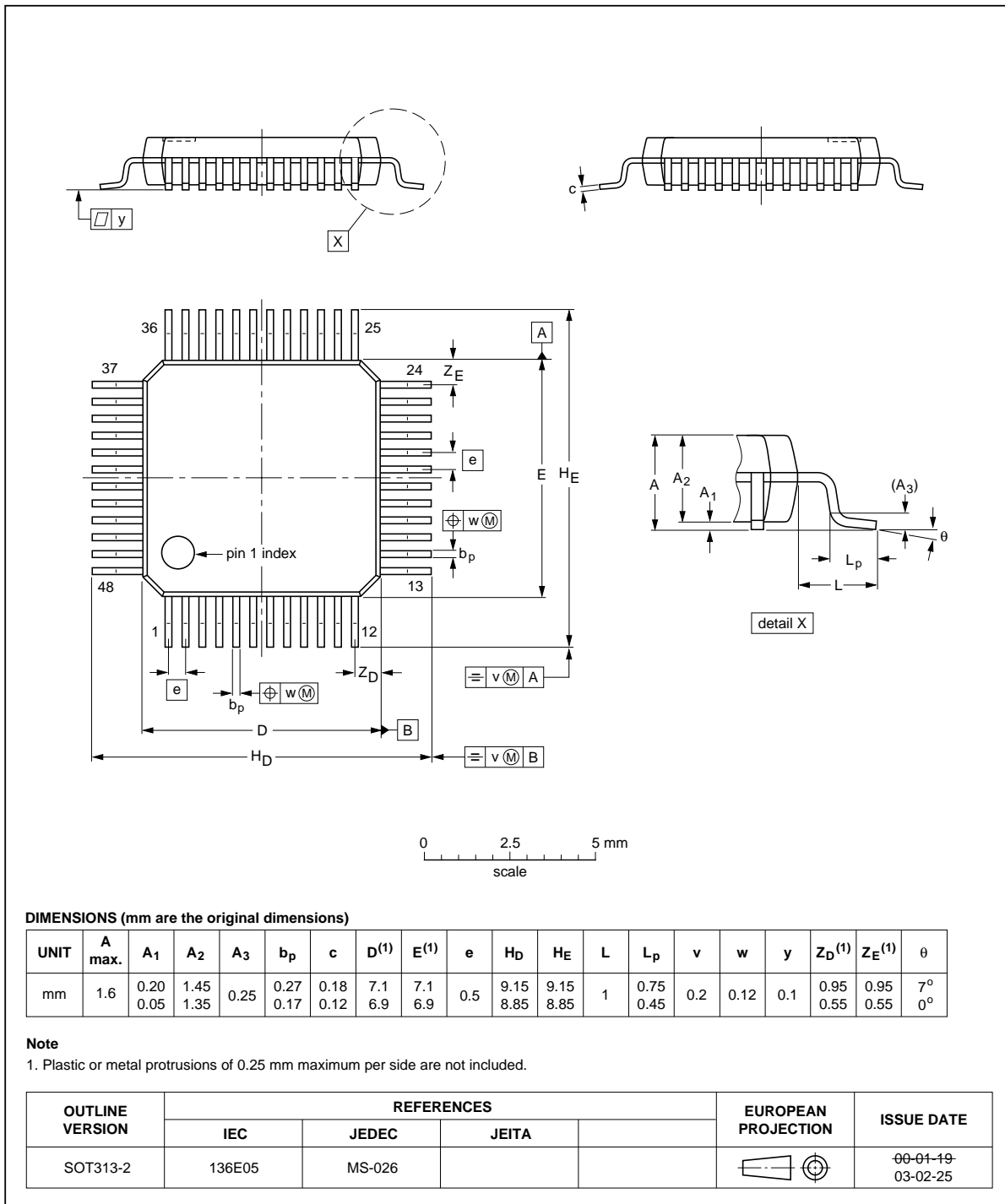
Fig 34. Package outline LQFP48
