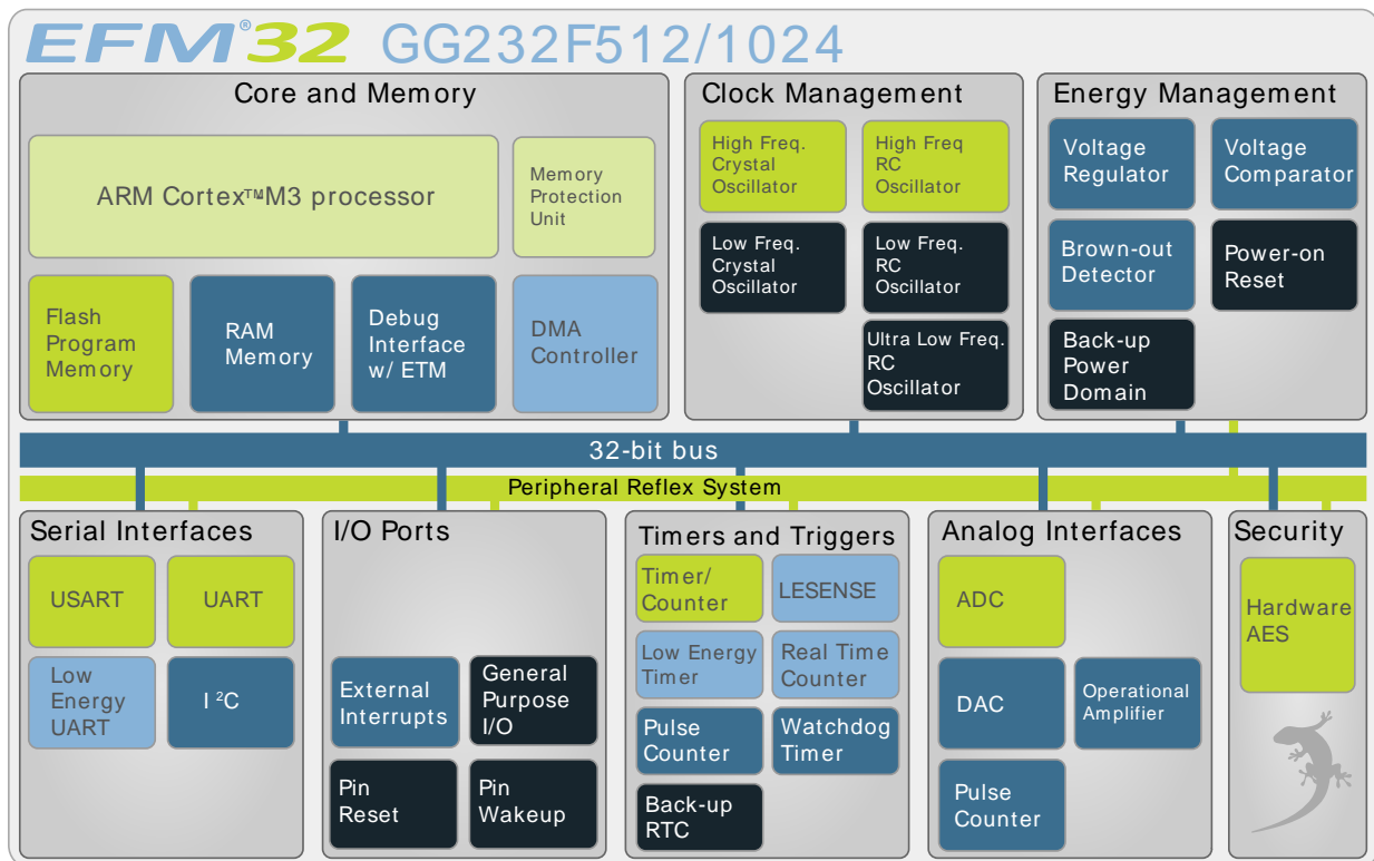
Figure 2.1. Block Diagram
