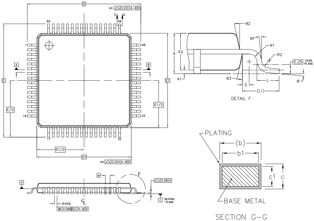
Figure 4.3. LQFP64
