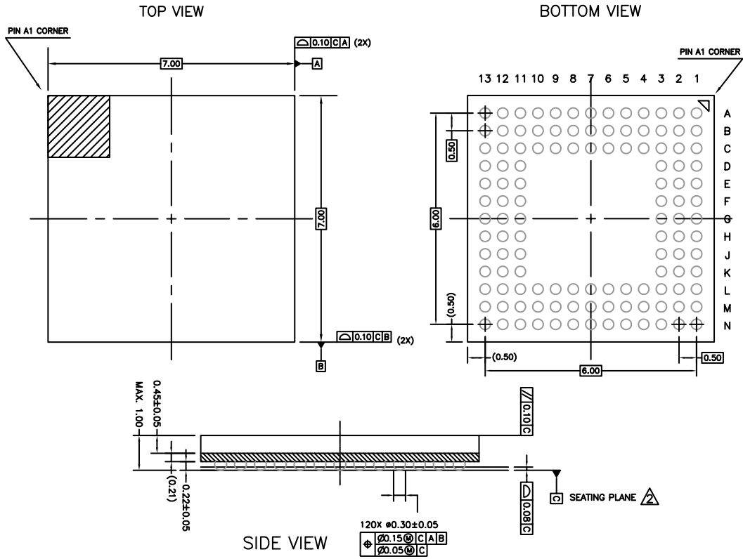
Figure 4.3. BGA120
