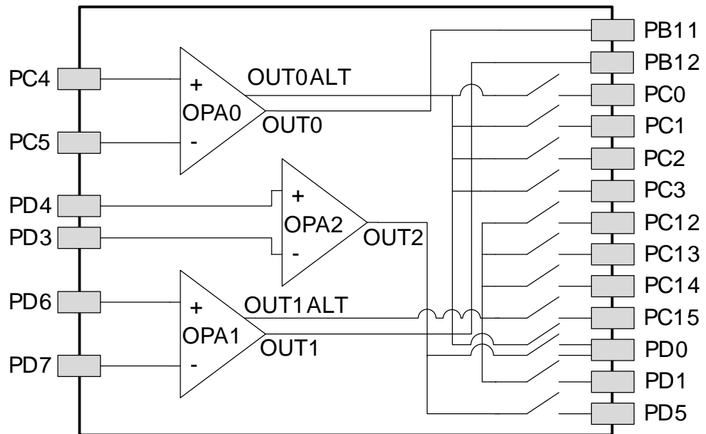
Figure 4.2. Opamp Pinout
