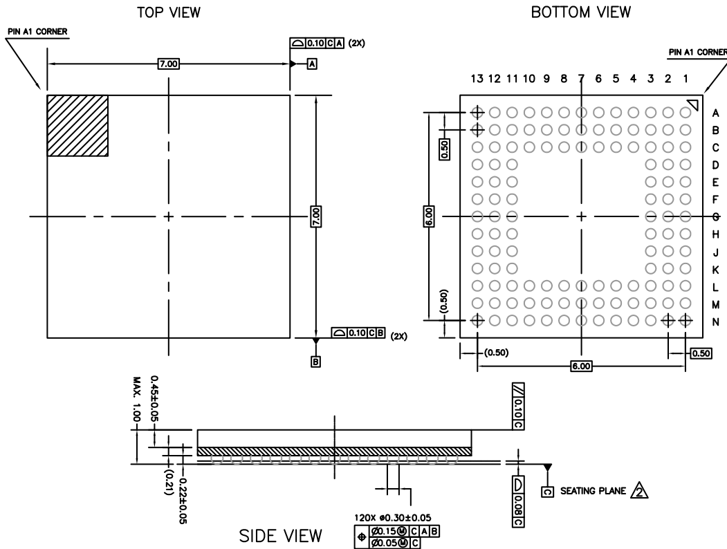
Figure 4.3. BGA120
