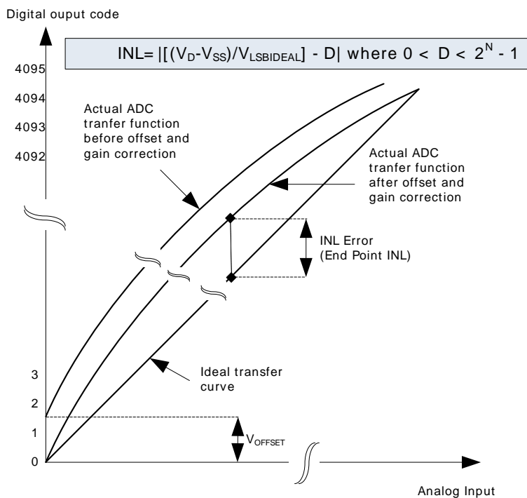
Figure 3.13. Integral Non-Linearity (INL)
