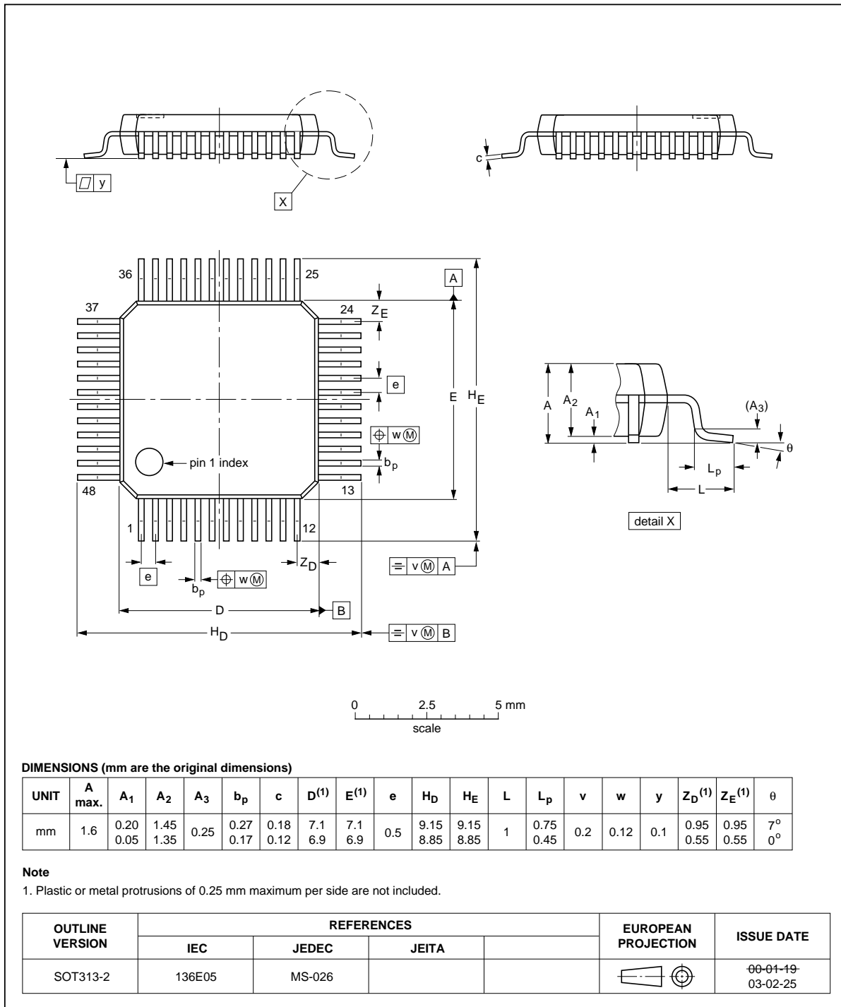
Fig 35. Package outline LQFP48 (SOT313-2)
