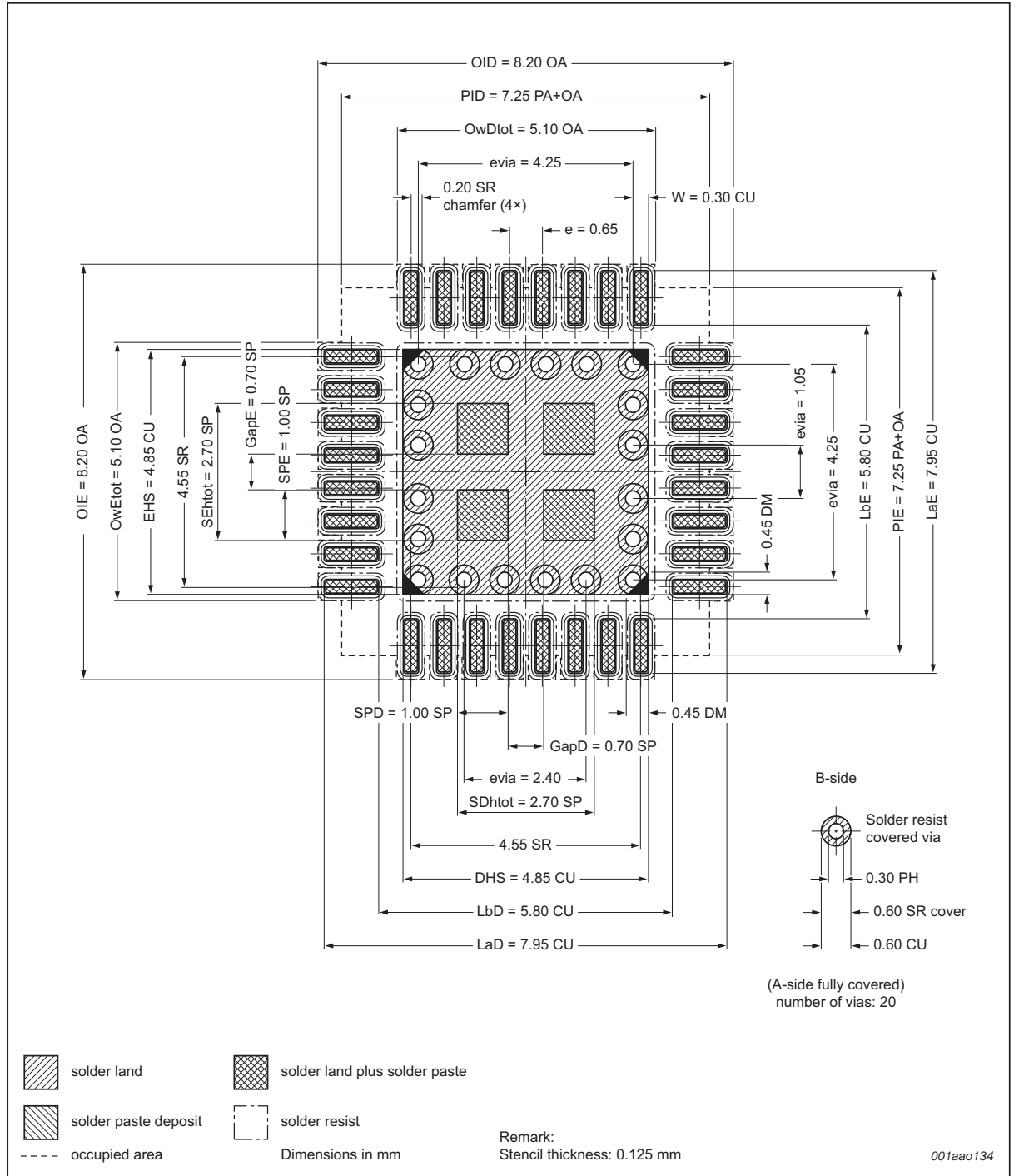
Fig 37. Reflow soldering of the HVQFN33 package
