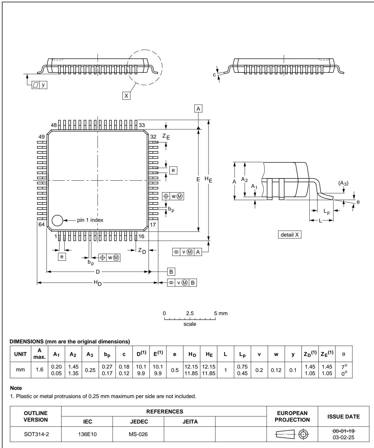
Fig 36. Package outline LQFP64 (SOT314-2)
