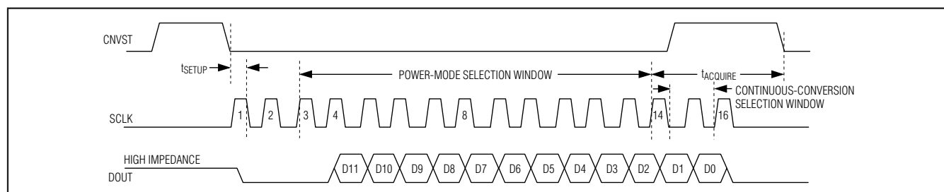
Figure 5. Interface-Timing Sequence
