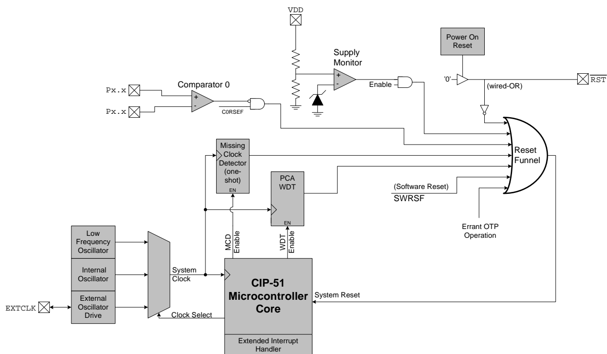
Figure 20.1. Reset Sources
