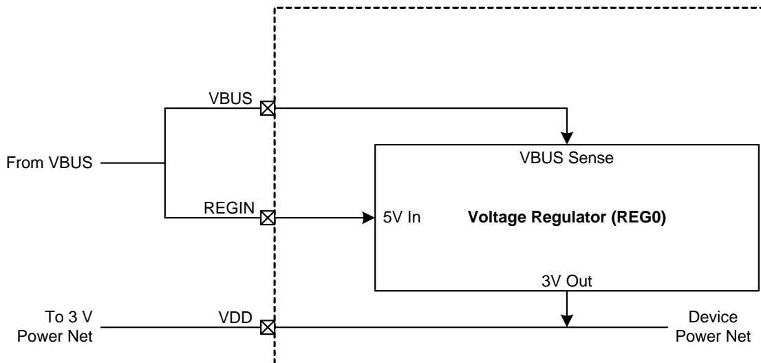
Figure 11.1. REG0 Configuration: USB Bus-Powered
