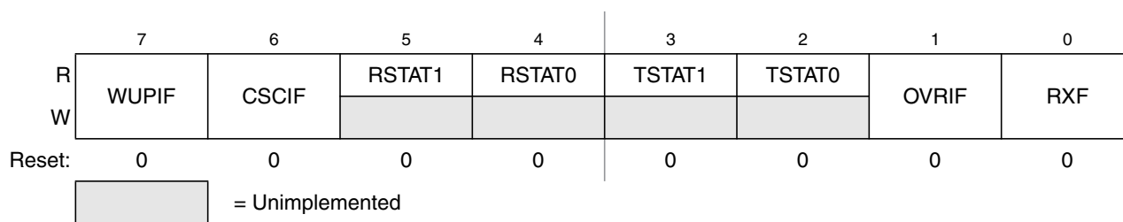
Figure 16-8. MSCAN Receiver Flag Register (CANRFLG)
