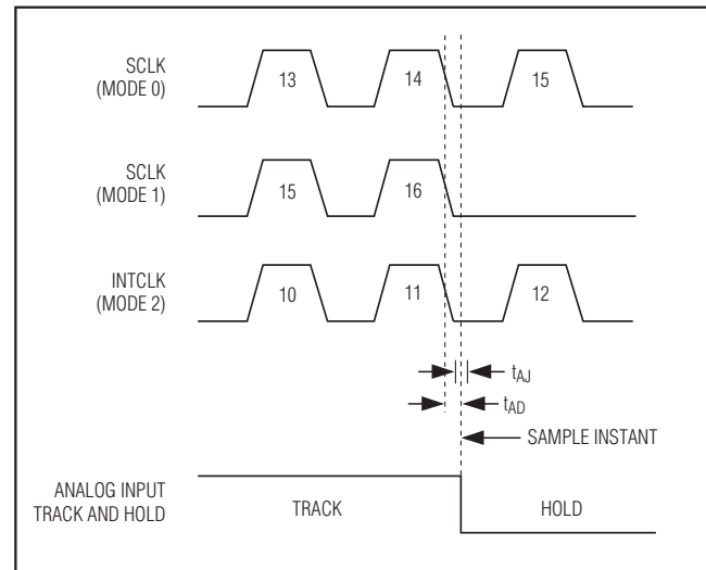
Figure 19. Aperture Diagram
