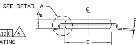
END VIEW
