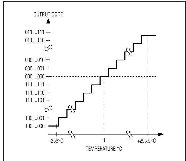
Figure 12. Temperature Transfer Function
