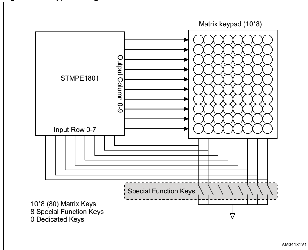
Figure 8. Keypad configuration
