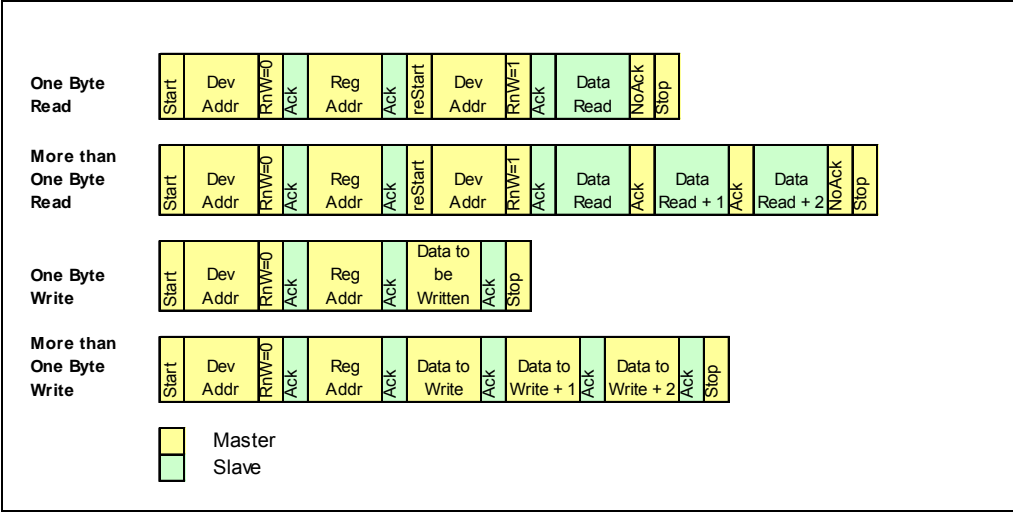
Figure 3. Operating modes
