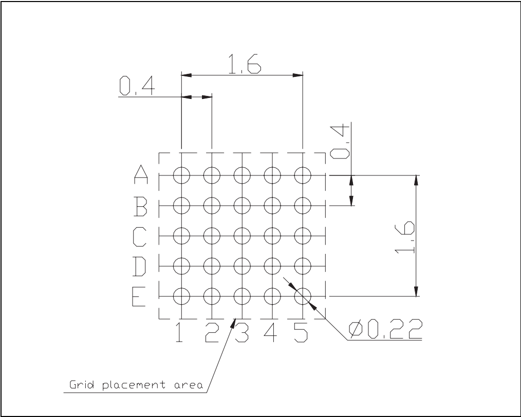
Figure 11. Footprint recommendation
