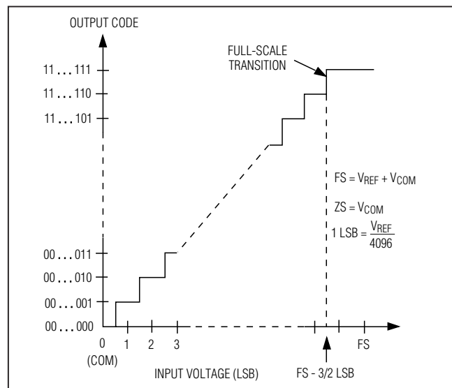
Figure 8. Unipolar Transfer Function, Full Scale (FS) = V_{\text{REF}}
