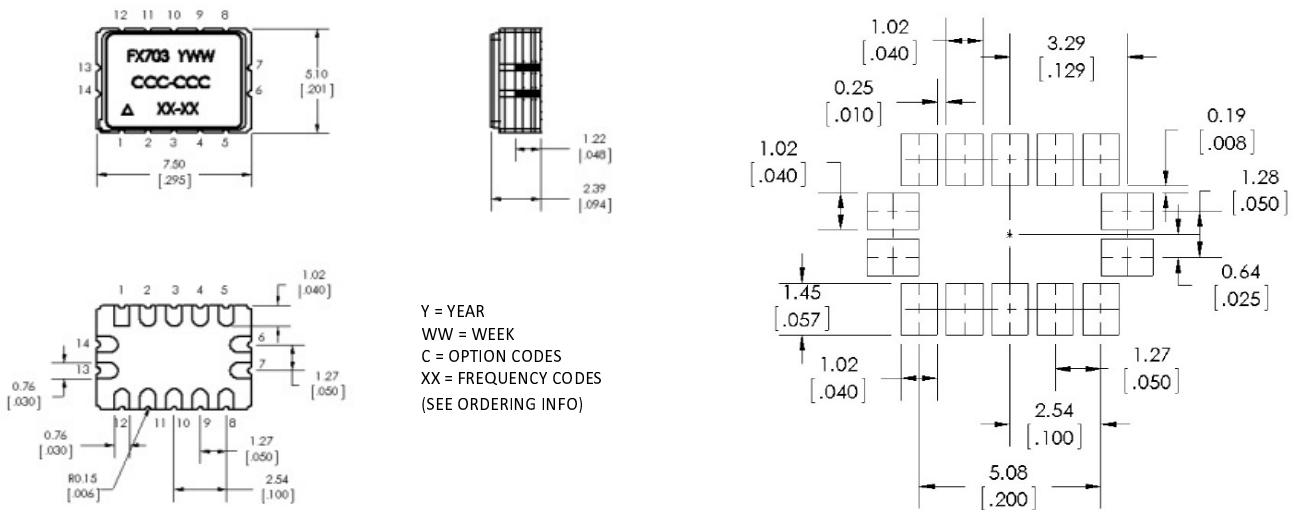
Figure 5. Outline Diagram & Suggested Pad Layout
