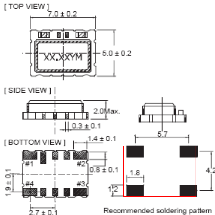
Figure 3, Package drawing
