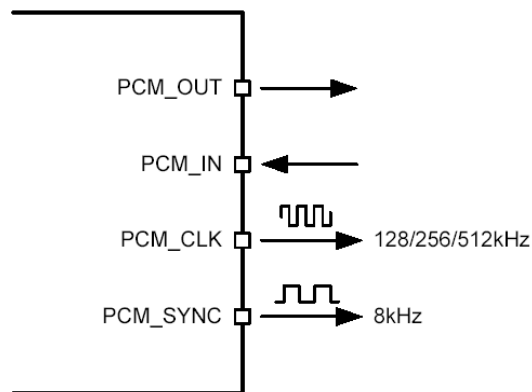
Figure 13: PCM Interface Master
