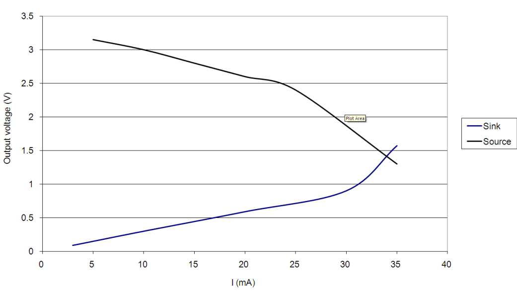
Figure 2: WT11i PIO Current Drive Capability
