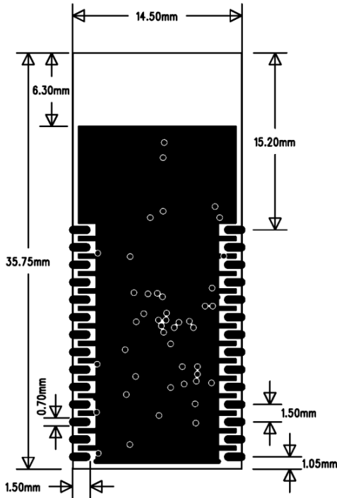
Figure 3: Physical dimensions (top view)
