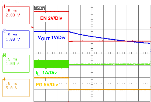
FIGURE 39. SOFT-DISCHARGE SHUTDOWN
