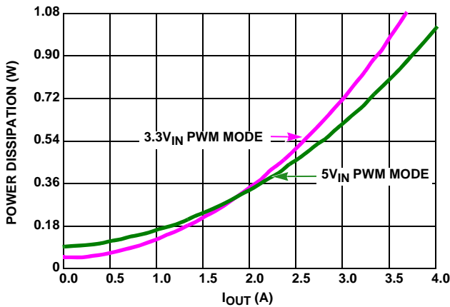
FIGURE 9. POWER DISSIPATION vs LOAD (1MHz, V OUT = 1.8V)
