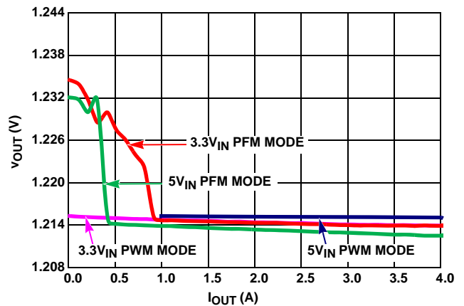
FIGURE 10. V OUT REGULATION vs LOAD (1MHz, V OUT = 1.2V)
