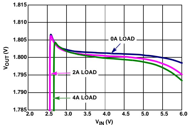
FIGURE 15. OUTPUT VOLTAGE REGULATION vs V_{IN} (PWM V_{OUT} = 1.8\text{V} )
